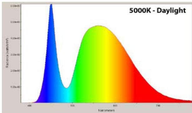
Light Output Intensity - Spectral Distribution
